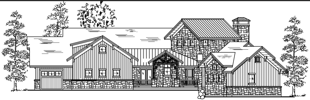
FRONT ELEVATION
