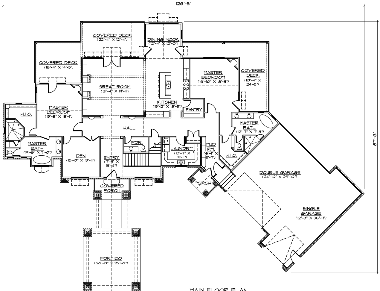
MAIN FLOOR PLAN (3316 SQ. FT.)
